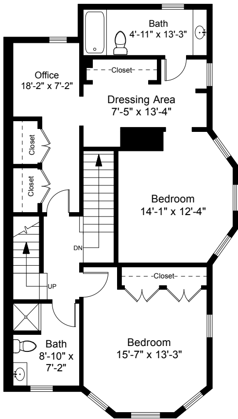
Second Floor Plan Ceiling Height = 8'-4"
