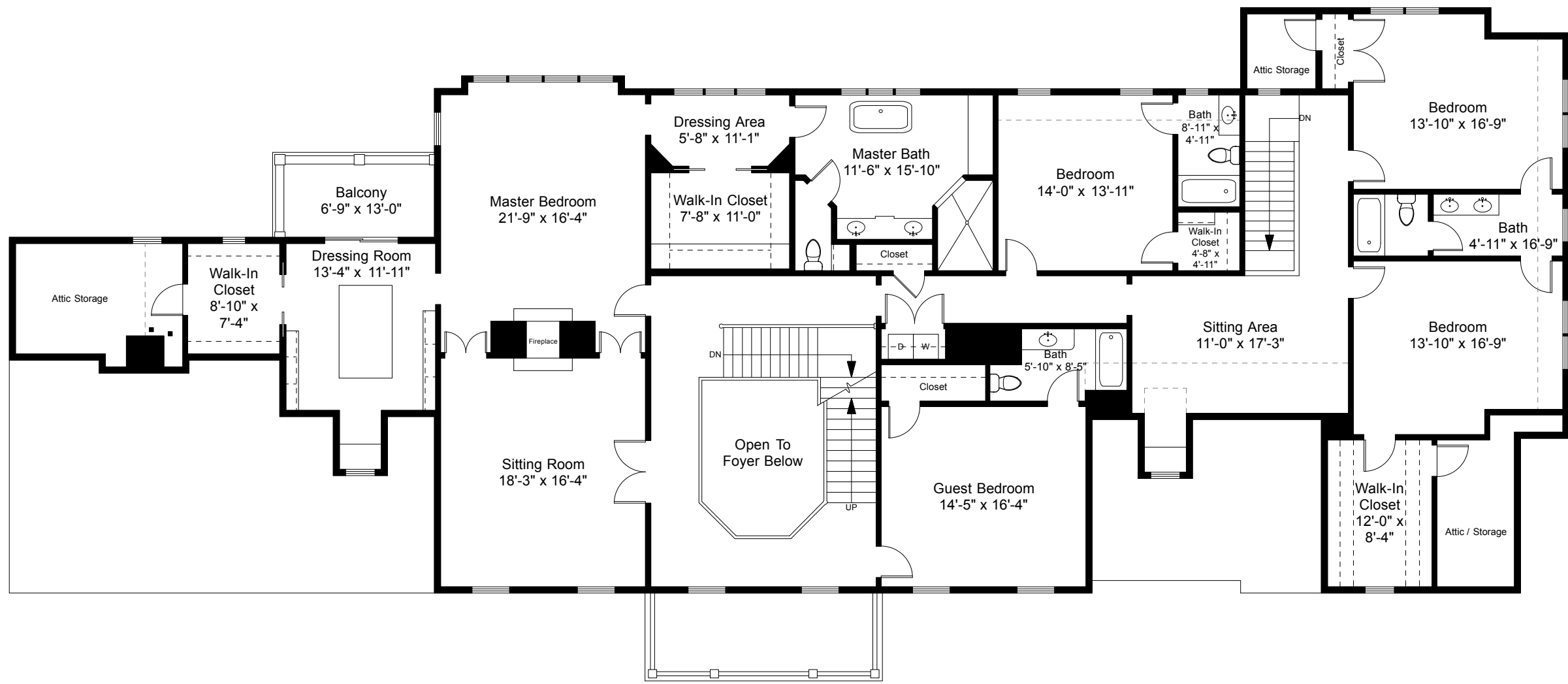
Second Floor Plan Ceiling Height = 8'-6"
