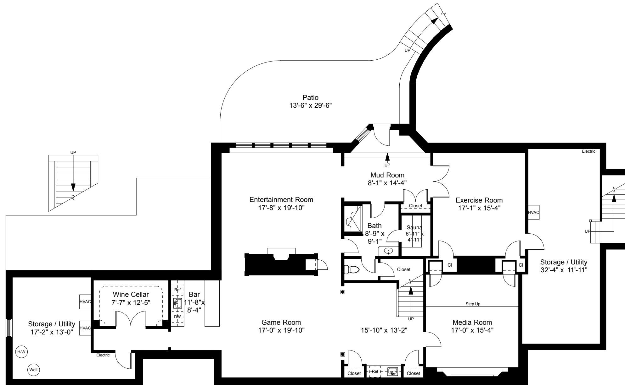
Lower Level Plan Ceiling Height = 8'-5"
