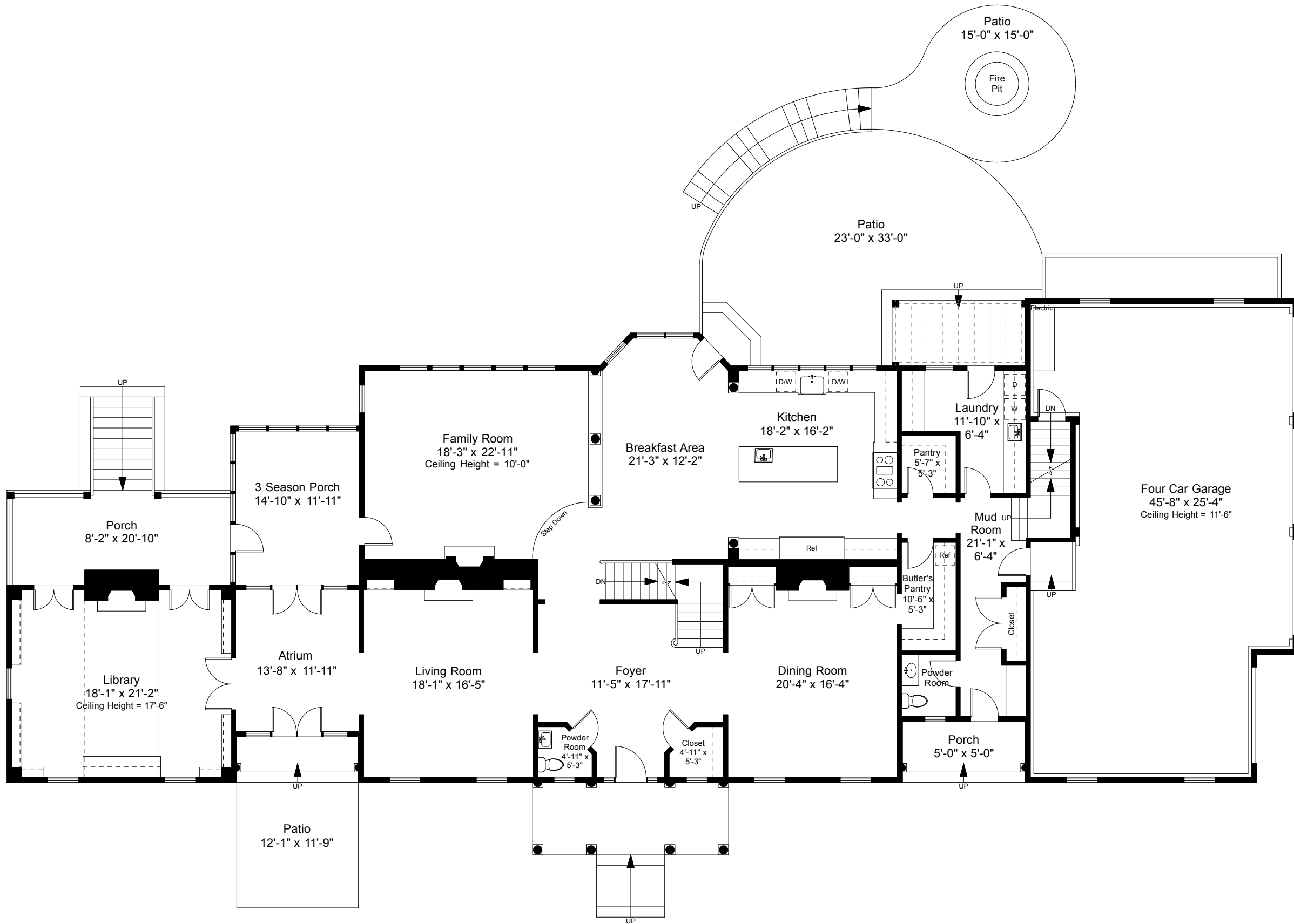
First Floor Plan Ceiling Height = 9'-6"
