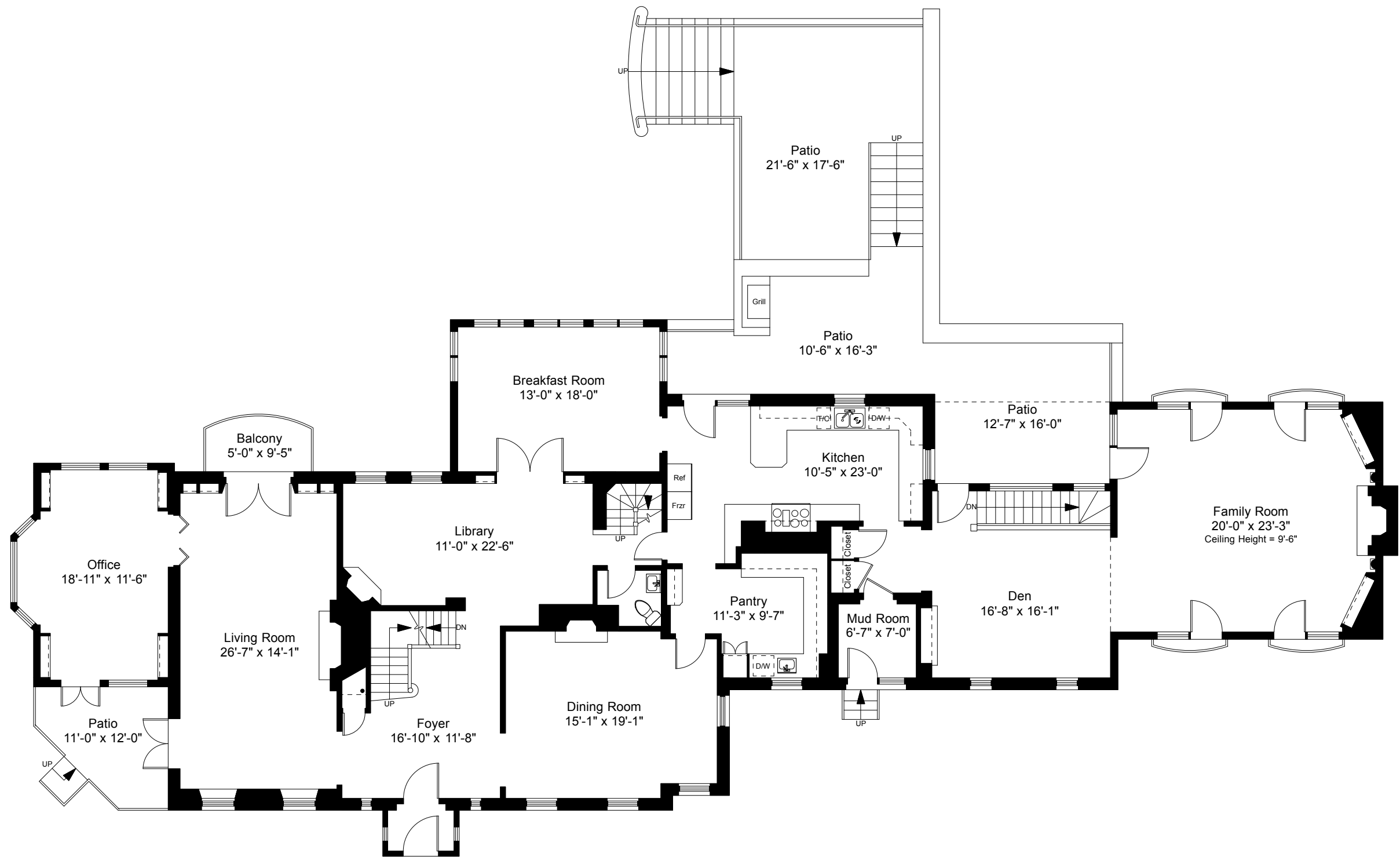
First Floor Plan Ceiling Height = 8'-0"
