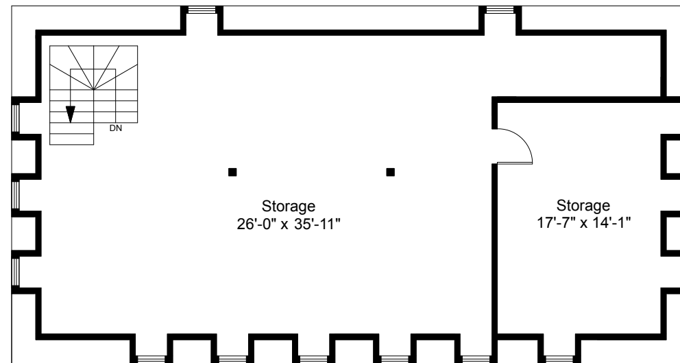
Carriage House - Second Floor Plan Ceiling Height = 8'-6"
