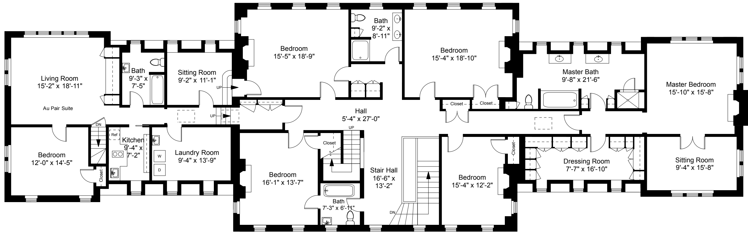
Second Floor Plan Ceiling Height = 8'-6"
