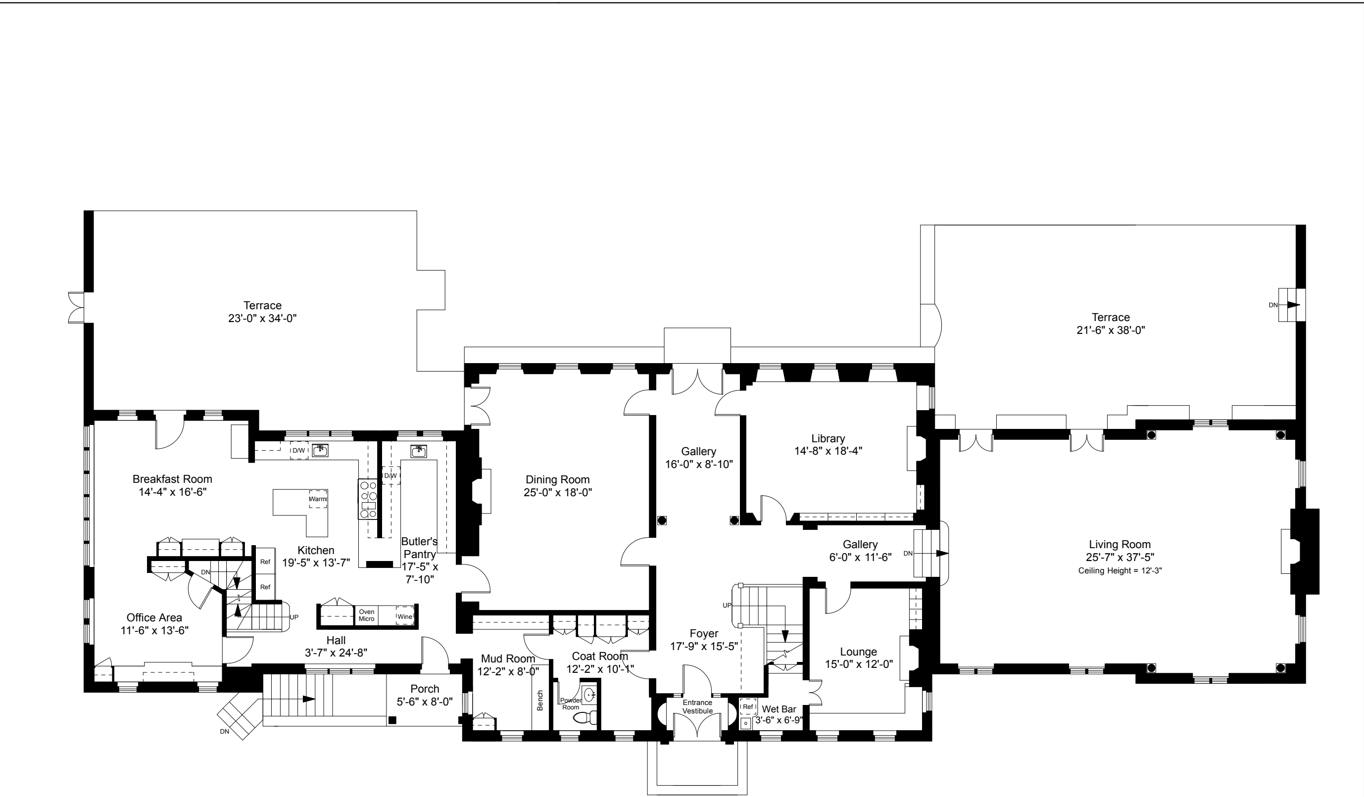
First Floor Plan Ceiling Height = 10'-0"
