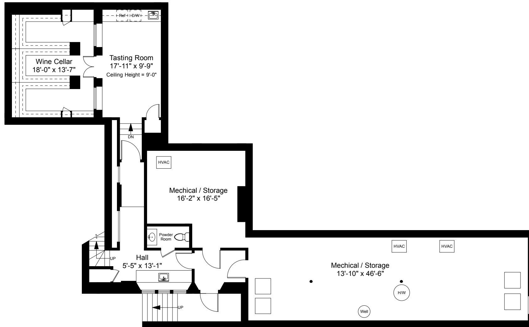
Lower Level Plan Ceiling Height = 7'-9"
