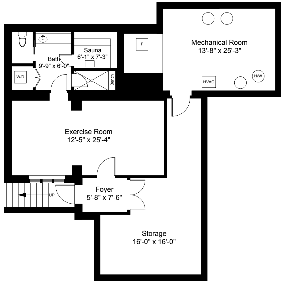
Pool House - Lower Level Plan Ceiling Height = 8'-5"
