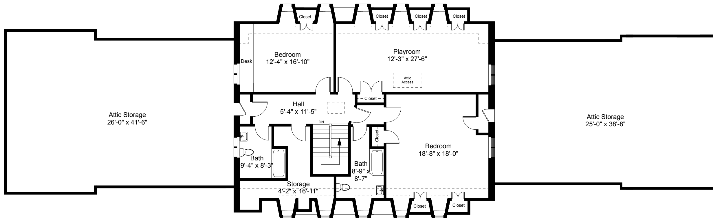
Third Floor Plan Ceiling Height = 8'-8"
