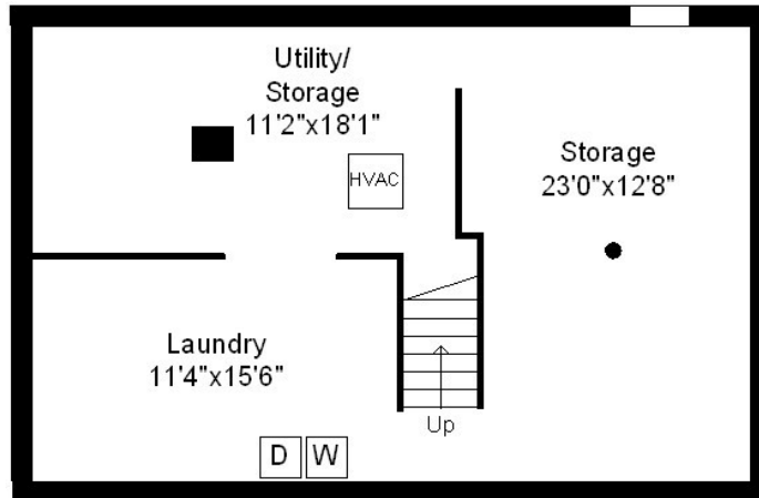
Basement Plan
