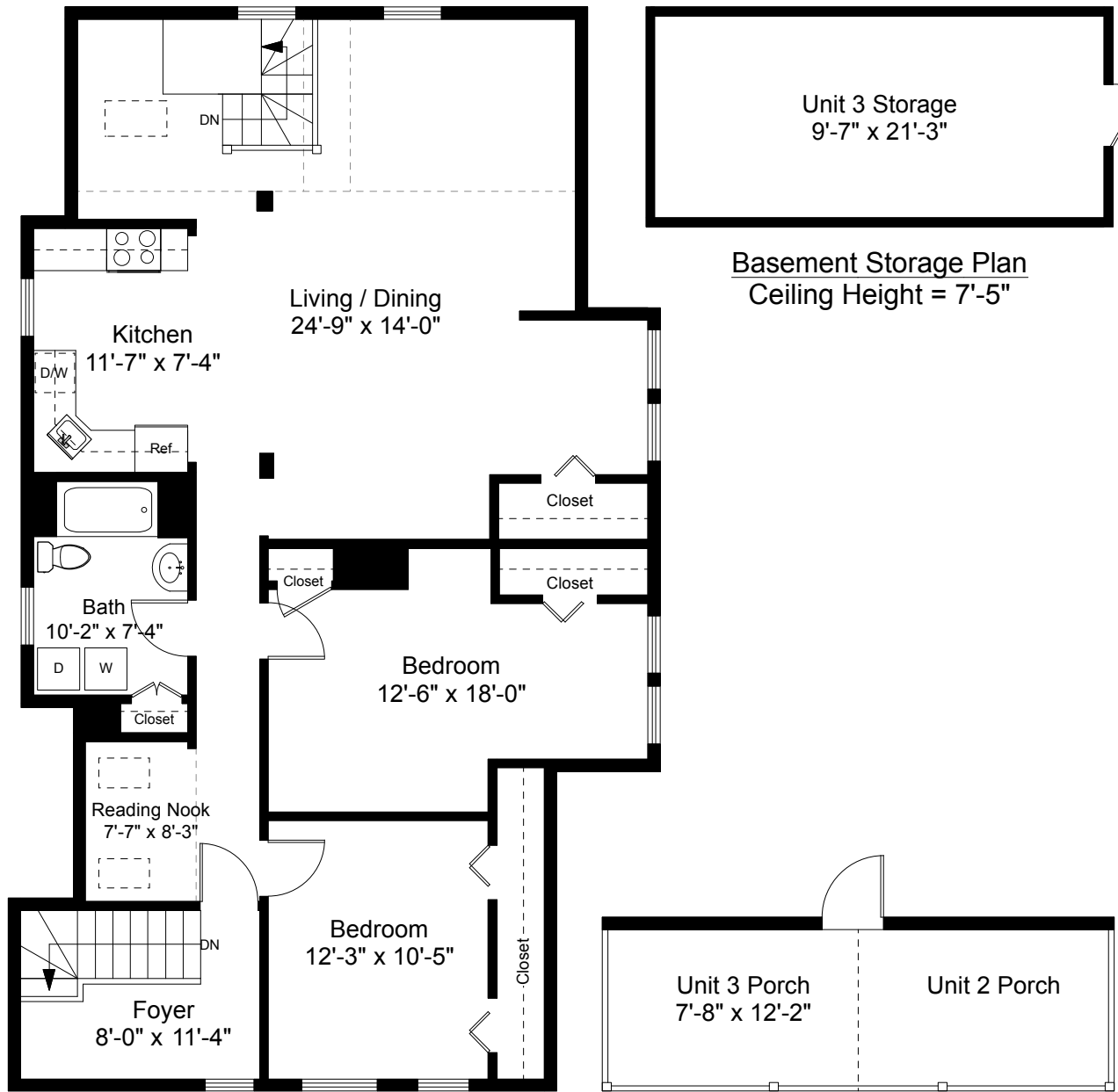
Unit 3 Floor Plan Ceiling Height = 8'-2"
