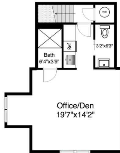
Garage - Second Floor Plan
