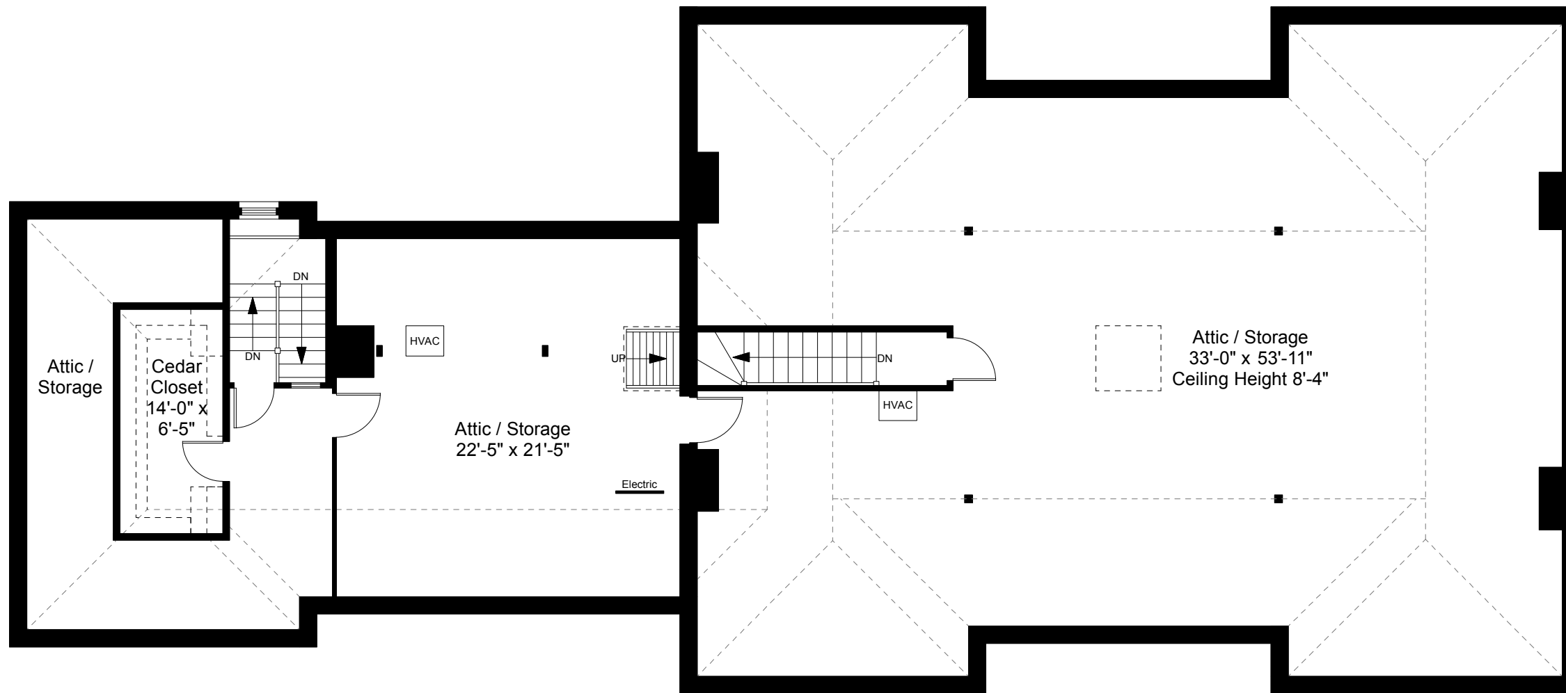
Third Floor Plan Ceiling Height = 7'-0"
