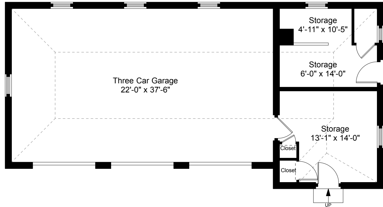
Garage Plan Ceiling Height = 18'-0"
