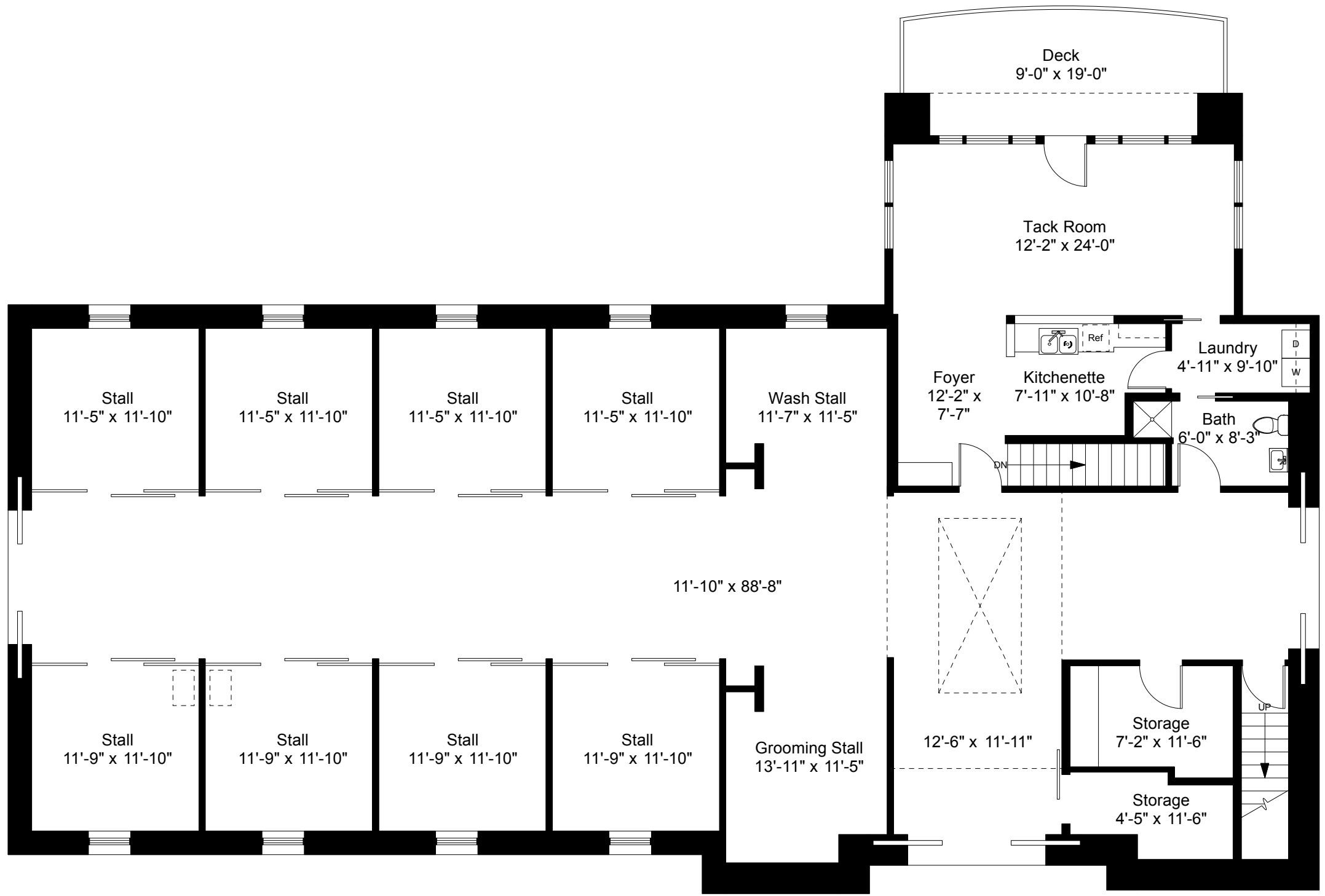
Stable - First Floor Plan Ceiling Height = 12'-0"
