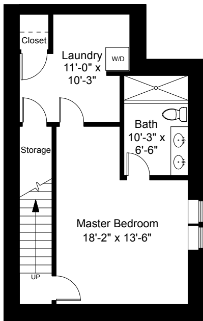
Lower Floor Plan Ceiling Height = 8'-1"
