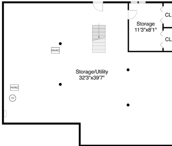
Basement Plan
