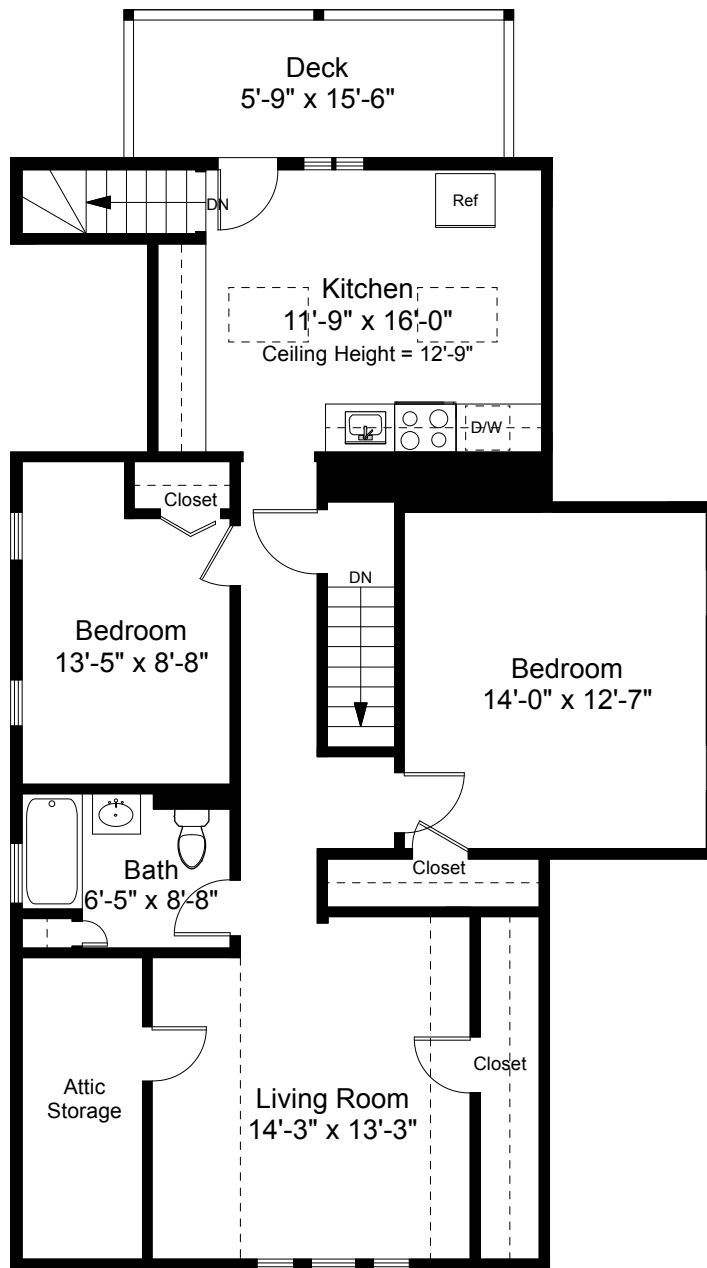
Unit 3 Floor Plan Ceiling Height = 7'-8"
